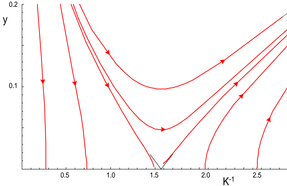
Figure 2: RNG flows for K^{-1} and y generated by numerical solutions of Eqs. (46) and (47).
