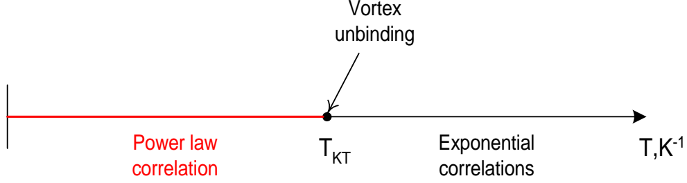
Figure 1: Schematic of the Kosterlitz-Thouless transition.
