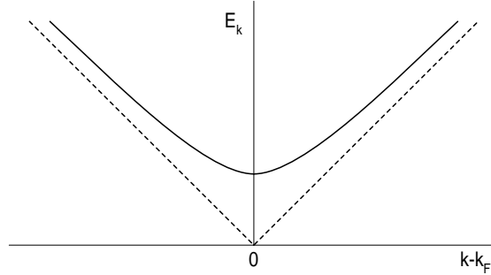
Figure 1: Excitation energy E_k for a BCS superconductor (solid line) and normal state (dashed line). The energy is defined as the cost to add a particle to a state \mathbf{k} with k > k_F relative to the chemical potential or to remove a particle from \mathbf{k} with k < k_F relative to -\mu . Thus the normal state spectrum is v_F |k - k_F| .
