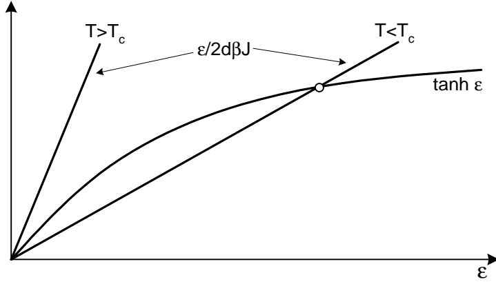
Figure 1: Graphical solution of the self consistency condition.
