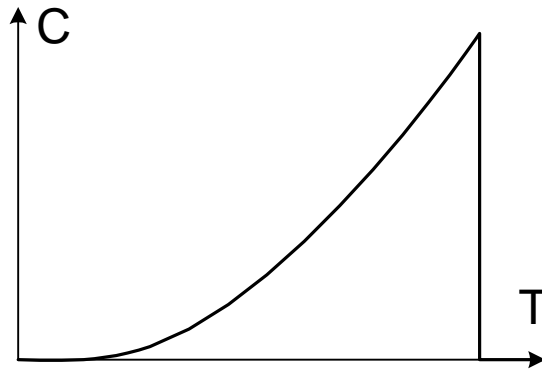
Figure 2: Specific heat of the Ising ferromagnet calculated in the mean field approximation.
