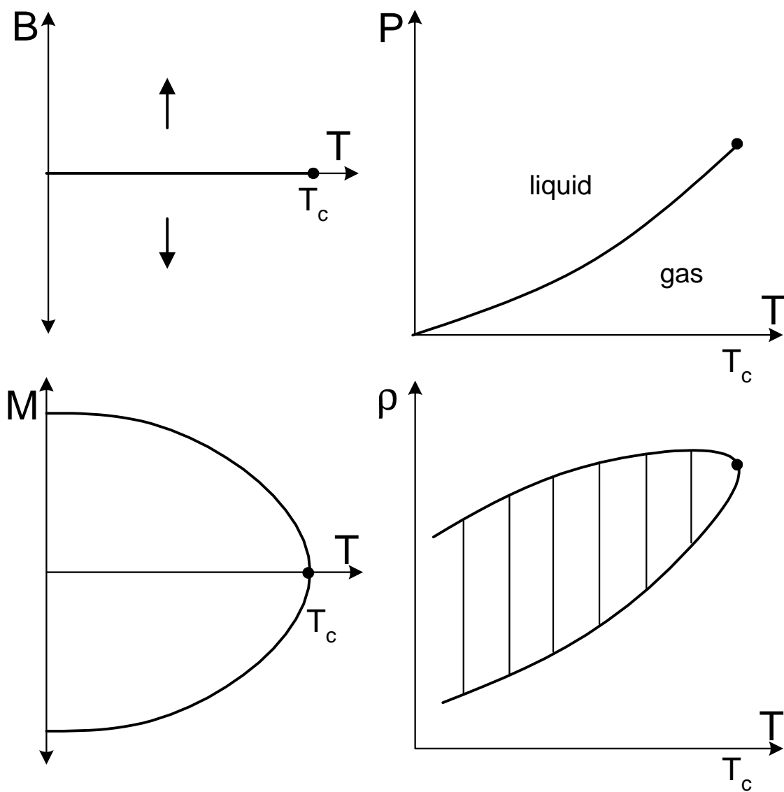
Figure 3: Analogy between Ising ferromagnet transition (left panels) and liquid-gas transition (right panels).
