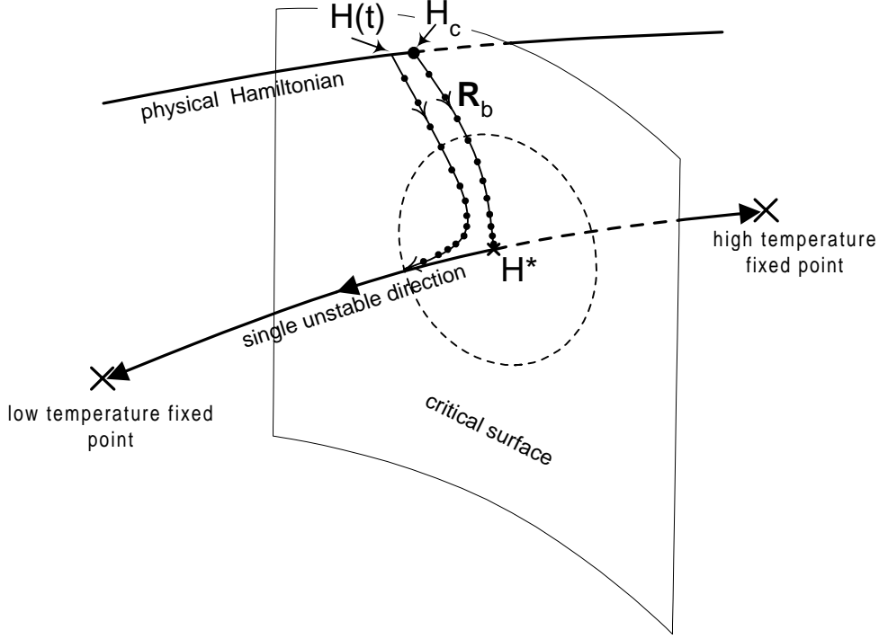
Figure 1: Flows near the critical surface
